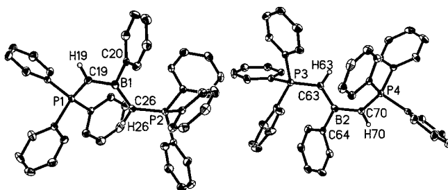
Figure 2. ORTEP drawings of two independent molecules of 2 . Thermal ellipsoids are at the 30 % probability level. Selected bond lengths [Å] and angles [°]: B1–C19 1.513(5), B1–C26 1.530(5), B1–C20 1.595(5), B2–C63 1.522(5), B2–C70 1.518(5), B2–C64 1.600(5), P1–C19 1.691(3), P2–C26 1.689(3), P3–C63 1.693(3), P4–C70 1.682(3), C19–B1–C26 124.1(3), C63–B2–C70 122.9(3).
