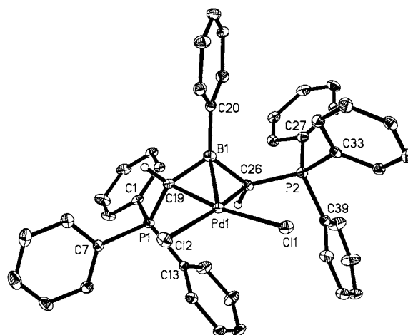
Figure 3. ORTEP drawing of complex 3 with thermal ellipsoids at the 30% probability level. Selected bond lengths [Å] and angles [ ^\circ ]: Pd1–C26 2.140(4), Pd1–C19 2.094(4), Pd1–B1 2.200(5), Pd1–Cl1 2.3705(11), Pd1–Cl2 2.3604, Cl1–Pd1–Cl2 93.45(4), P1–C19–Pd 112.8(2), P2–C26–Pd 128.8(2).
